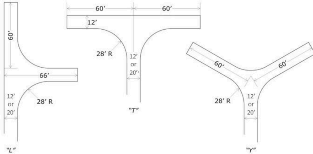
Figure 66-83 (3) Turn Around Options
