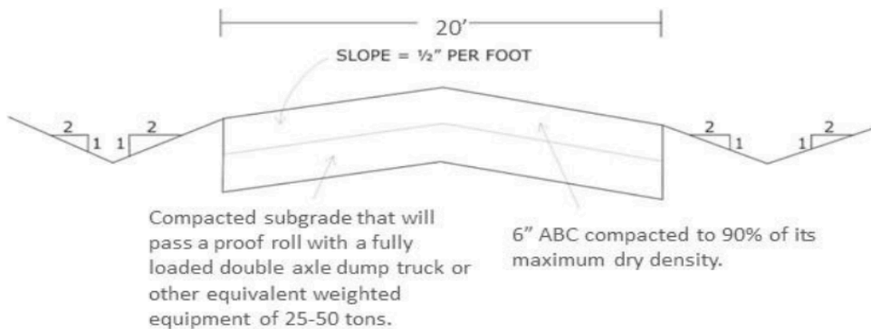
Figure 66-83 (1) Minimum All-Weather Path Standard
